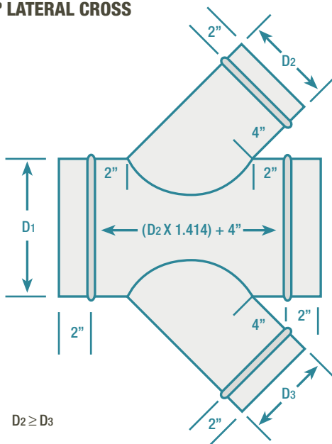
45° LATERAL CROSS
